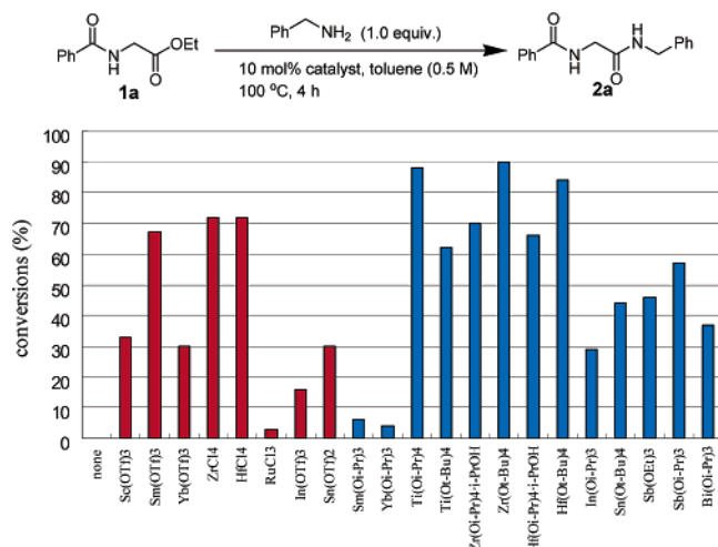
Figure 1. Results of catalyst screening for ester–amide exchange using benzylamine and ethyl hippurate. Conversion based on ^1\text{H} NMR analysis of the crude reaction mixture.
